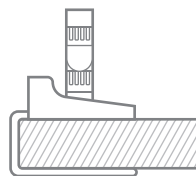
TOP DOWN CLAMP
